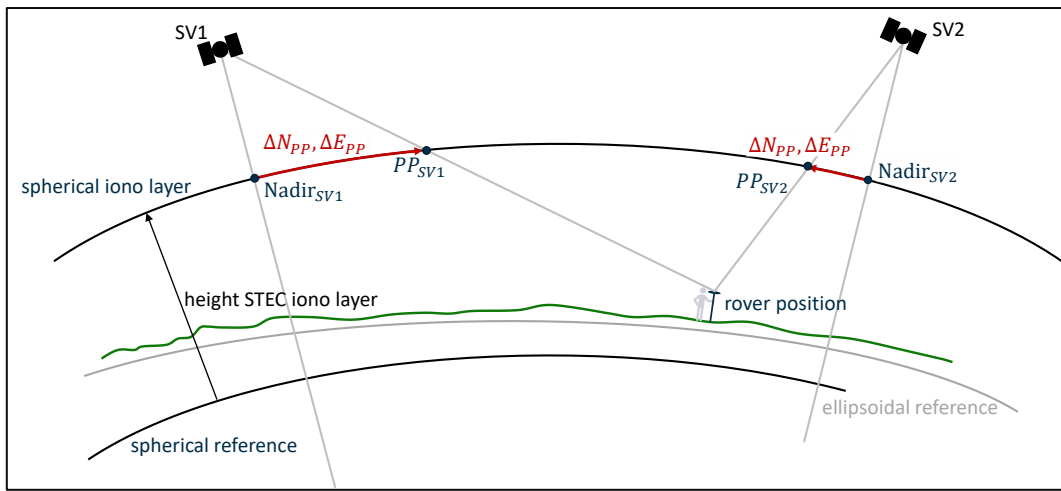
Figure 5 Pierce point origin of the GSI model. The PPO is defined by the nadir with respect to spherical layer.
